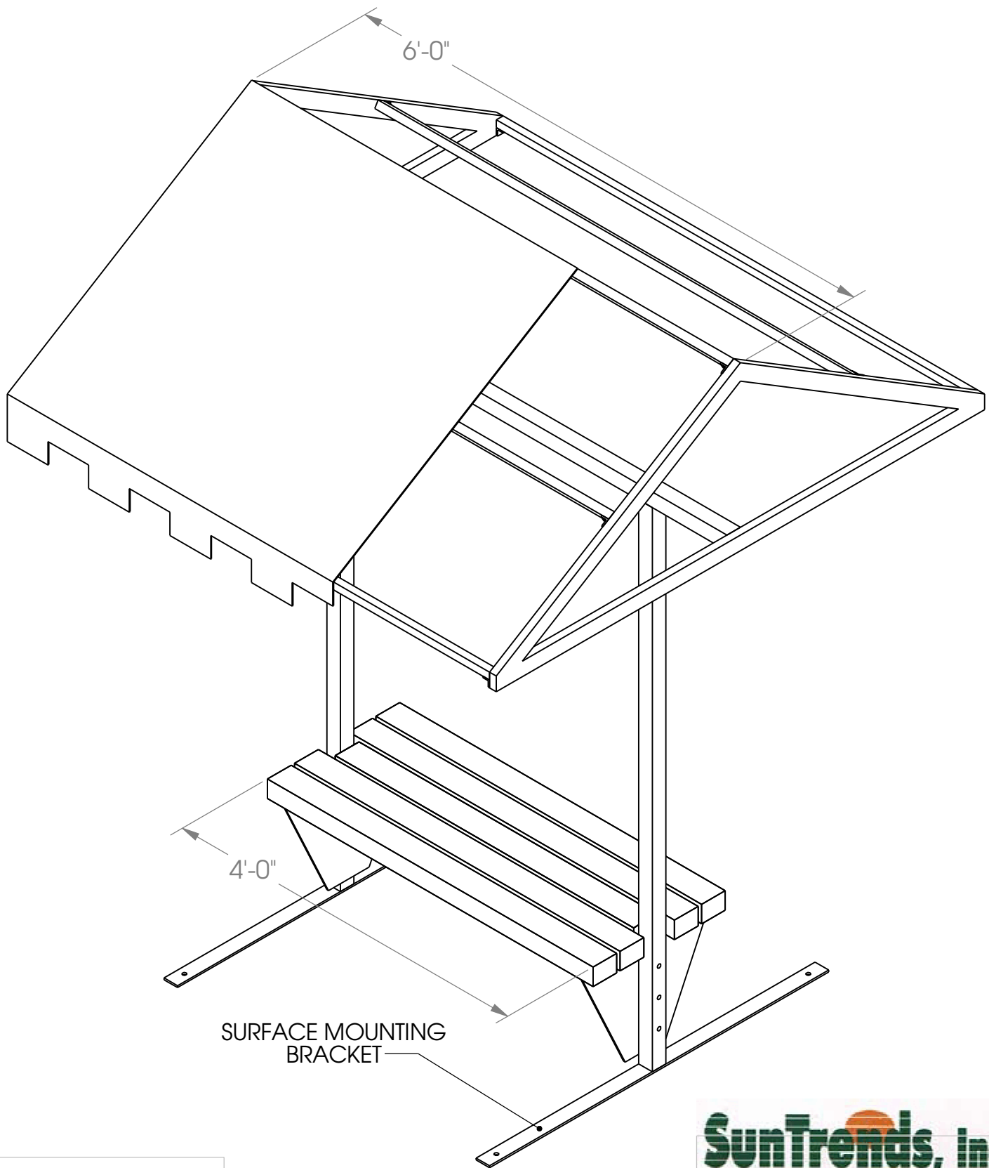
ISOMETRIC VIEW
