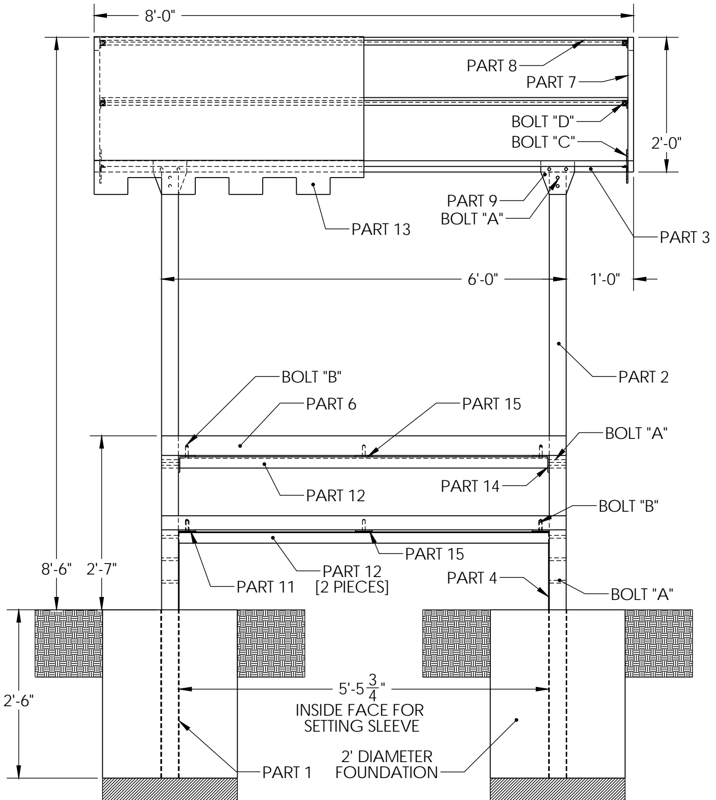
FRONT VIEW
