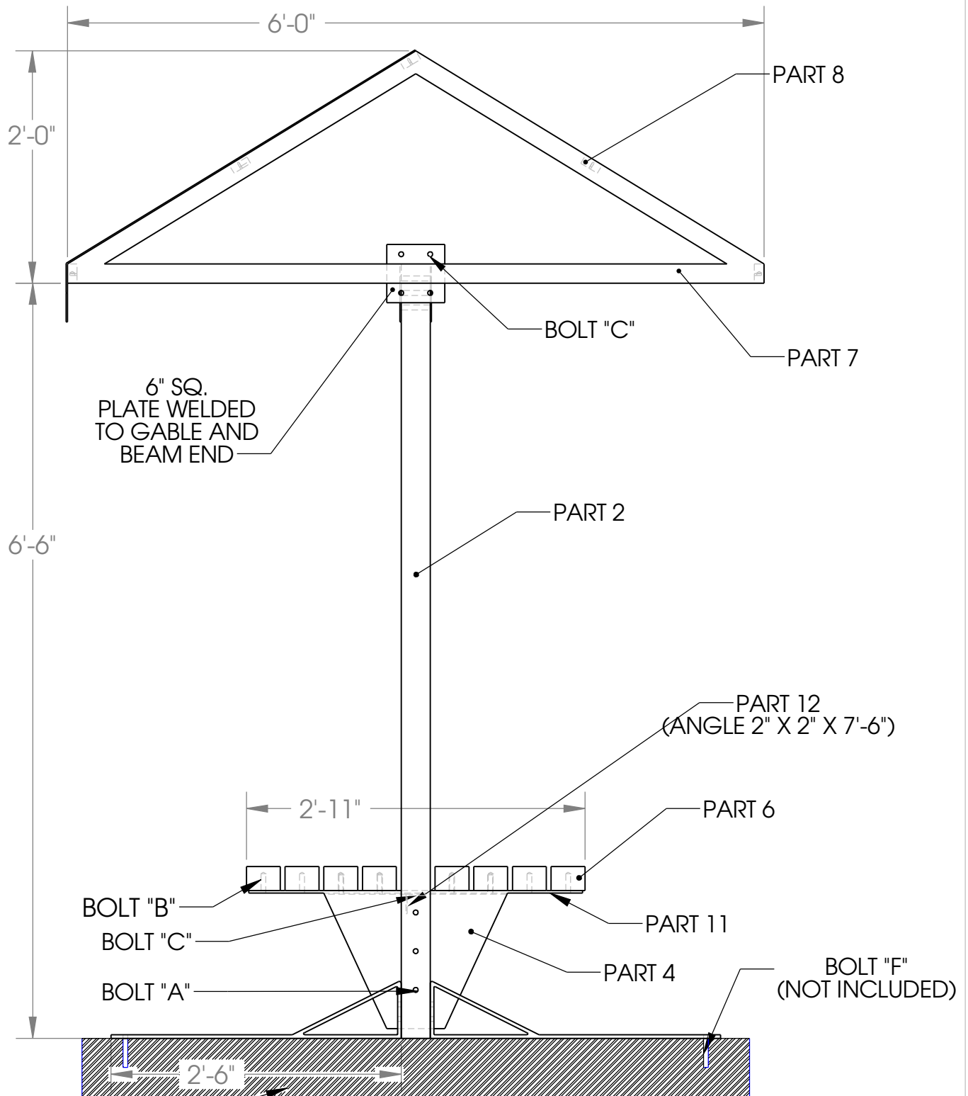
SIDE VIEW
